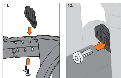
1.1. Screw the adapter onto the mudguard in keeping with the required hole pattern. Use the enclosed self-tapping screws for this. (TX20)
